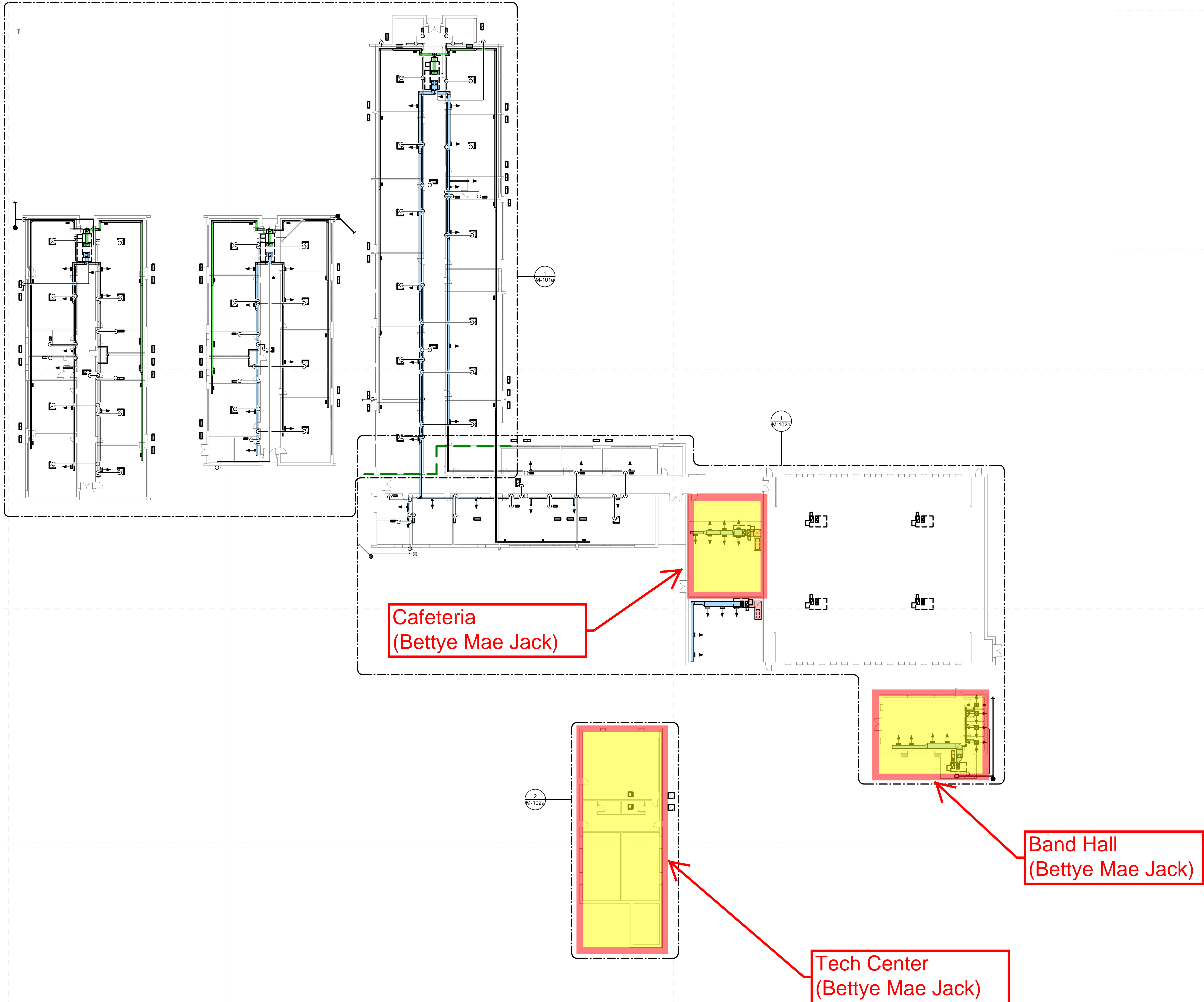
Bettye Mae Jack - New Work Overall Mechanical Plan 1 M-001a 1" = 20'-0"
